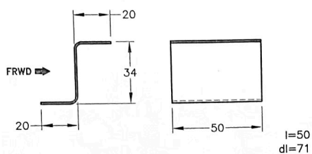
2 VALVE REAR SUPPORT t=.032" 6061-T6 (1 REQ'D)
