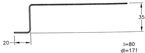
1 VALVE MAIN SUPPORT t=.032" 6061-T6 (1 REQ'D)
